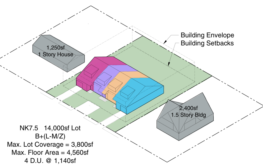
NK7.5 B+(L-M/Z) B = 2,500sf, Z = 5, 1.2 Ratio
