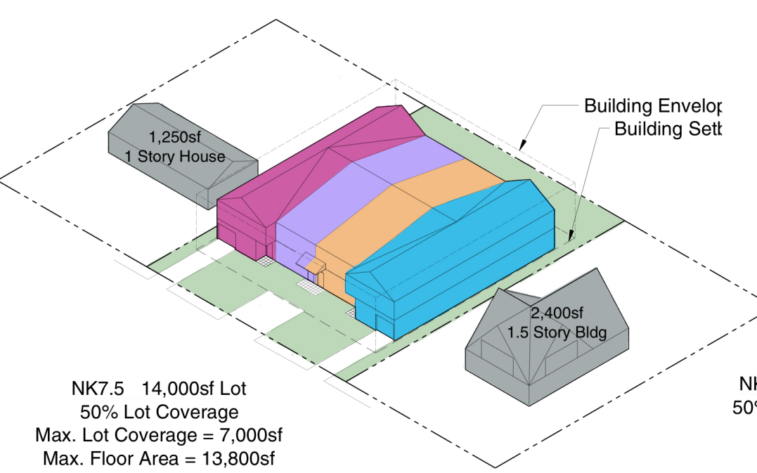
NK7.5 50% Lot Coverage
