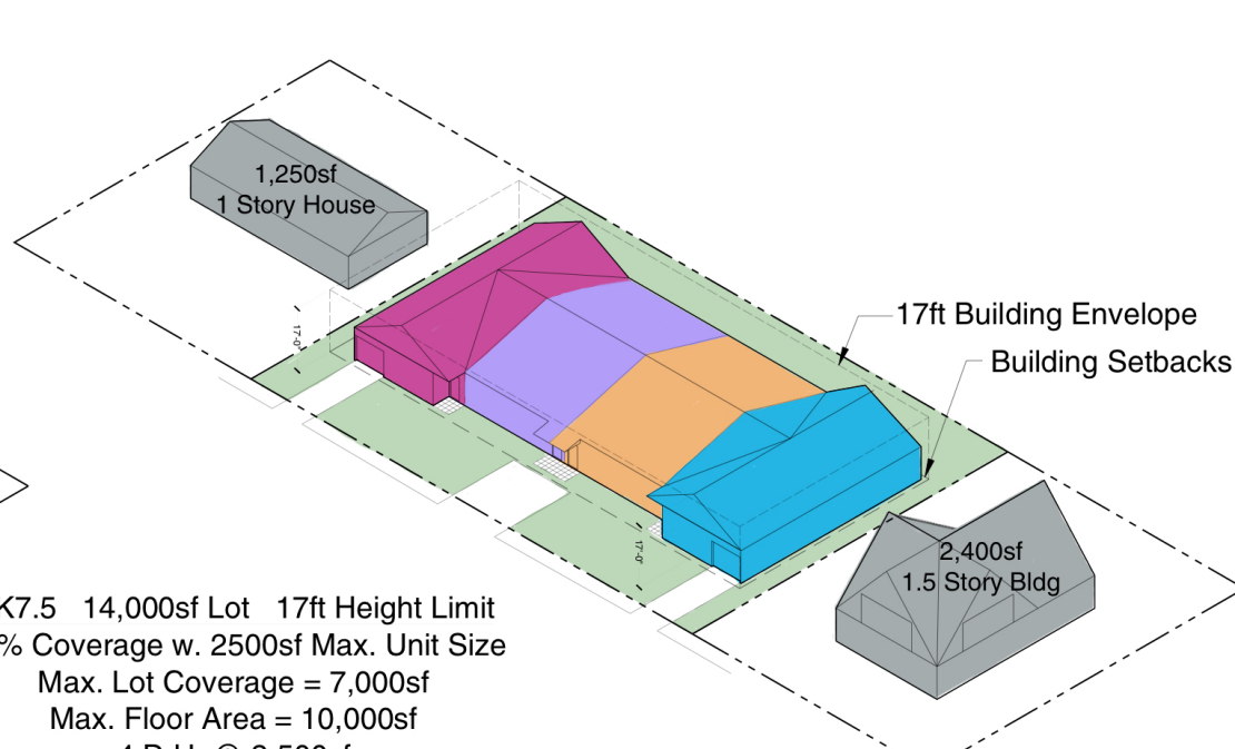
NK7.5 17ft Height Limit 50% Lot Coverage w/ 2500sf Max. Unit Size
