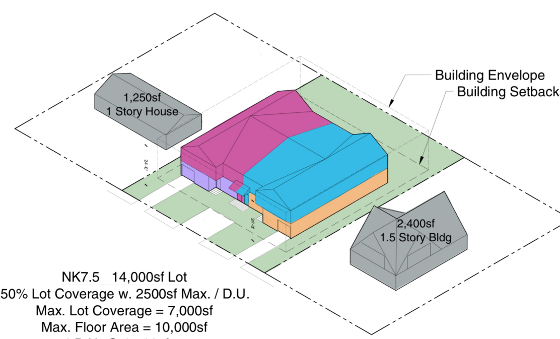
NK7.5 50% Lot Coverage w/ 2500sf Max. Unit Size
