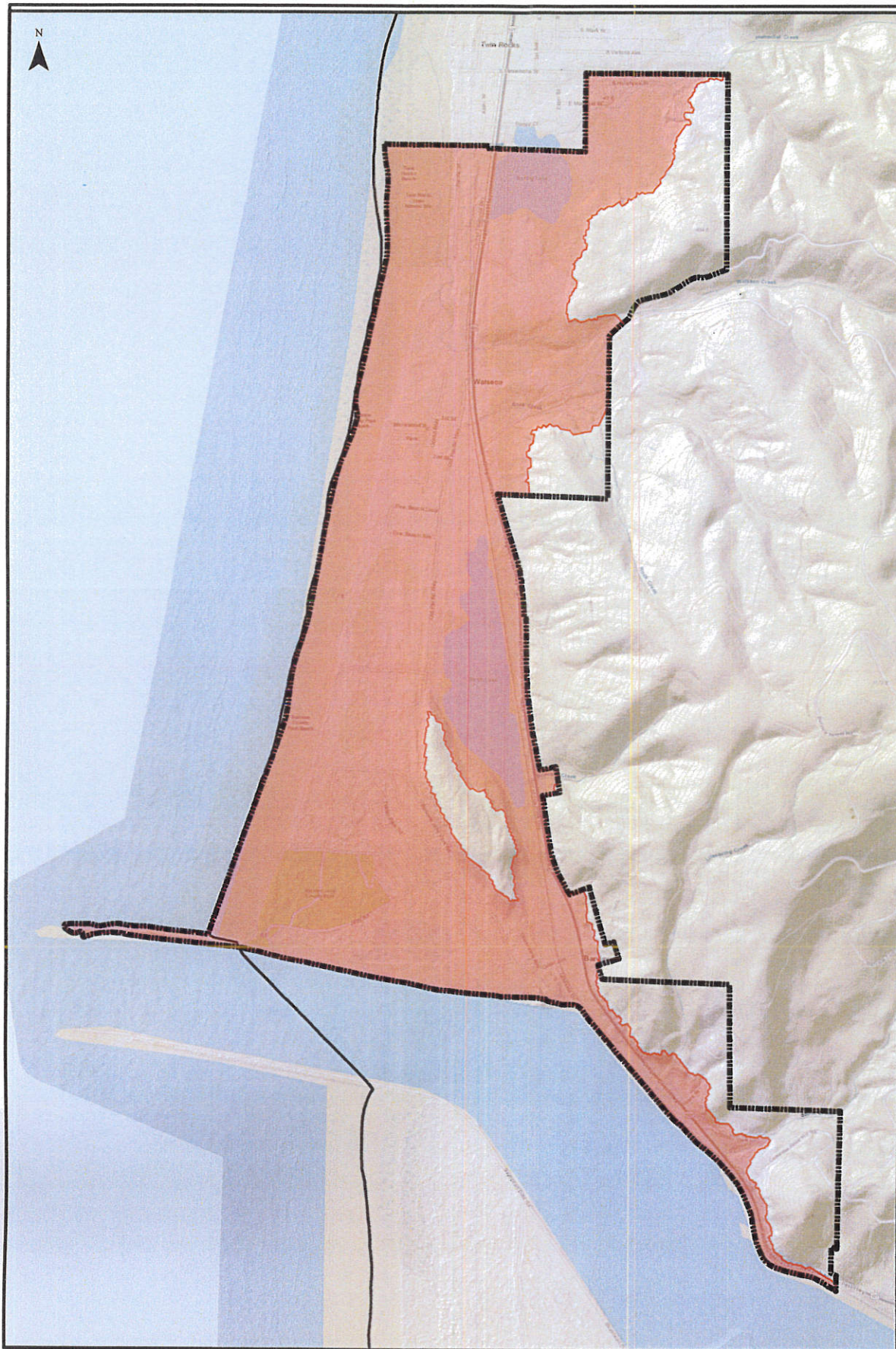
BARVIEW/WATSECO/TWIN ROCKS TSUNAMI INUNDATION ZONE: DOGAMI TIM XXL (100% potential variability CSZ)
